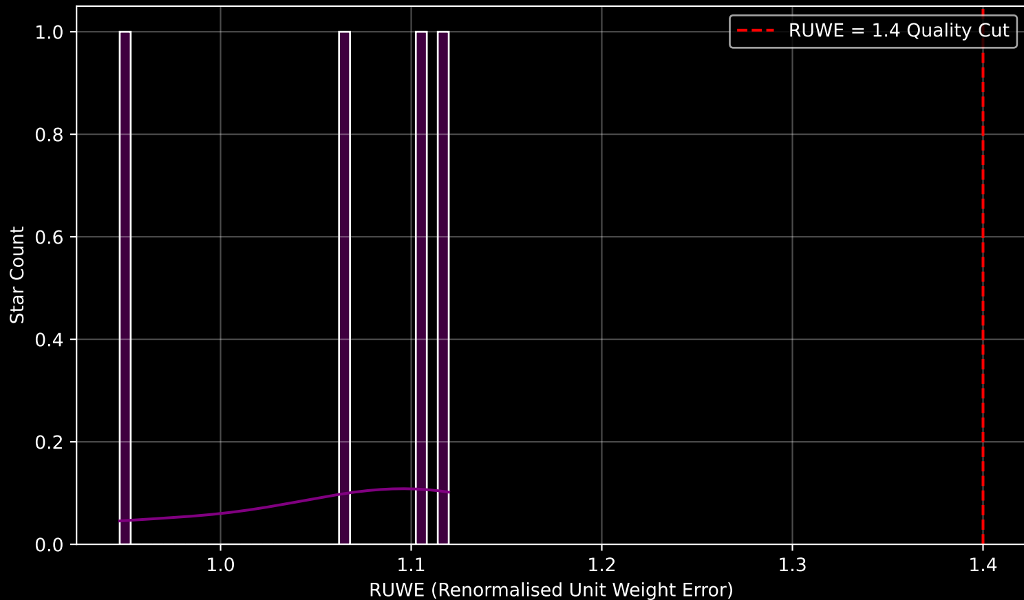
GAPOGEE DR17 Field [ruprecht147] RUWE Distribution (n= 4)
