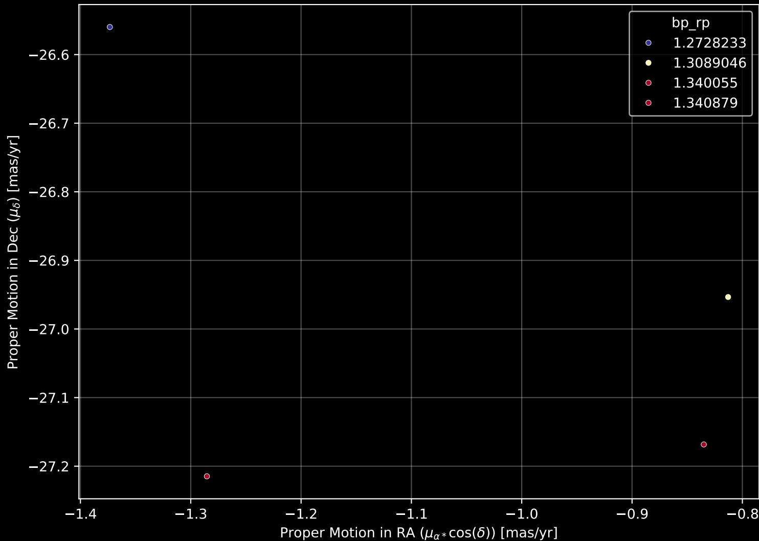
APOGEE DR17 Field: [ruprecht147] Proper Motion Diagram (n= 4)
