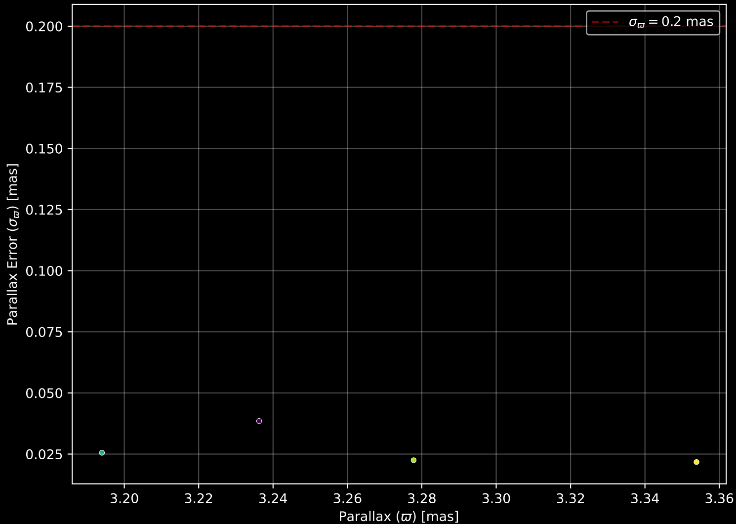
APOGEE DR17 Field: [ruprecht147] Parallax Quality (n= 4)
