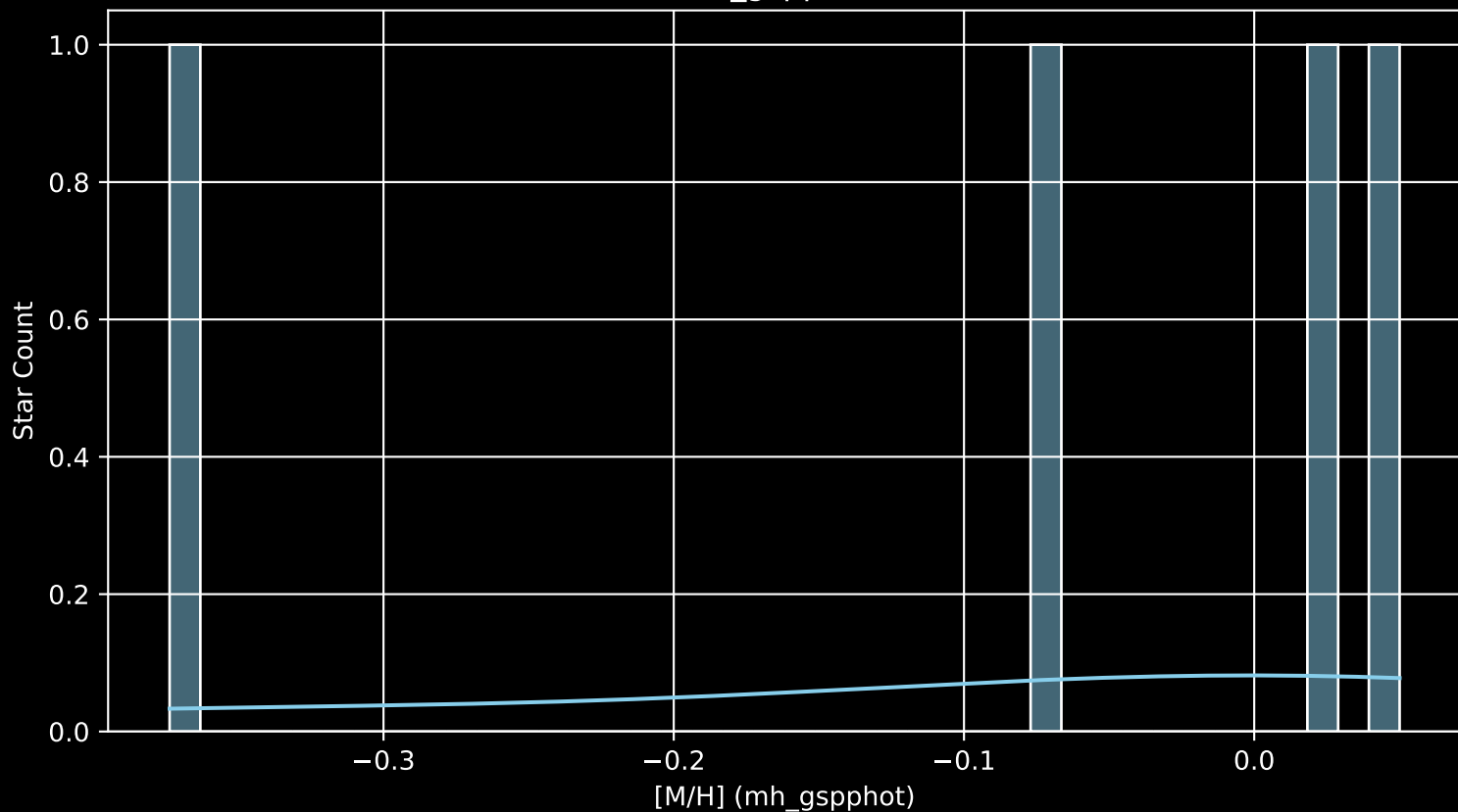
APOGEE DR17 Field: [ruprecht147 [M/H] (mh_gspphot) (n= 4)
