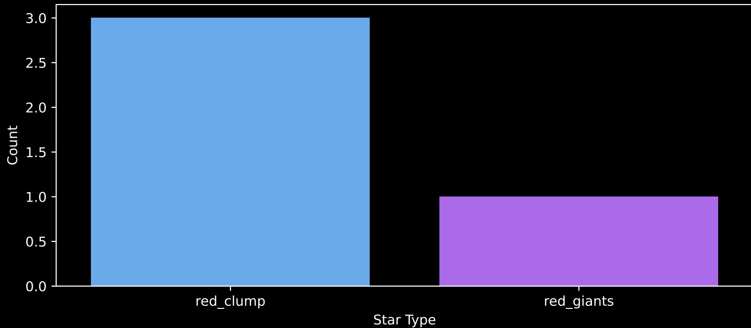
APOGEE DR17 Field: [ruprecht147] Count plot of Star Type
